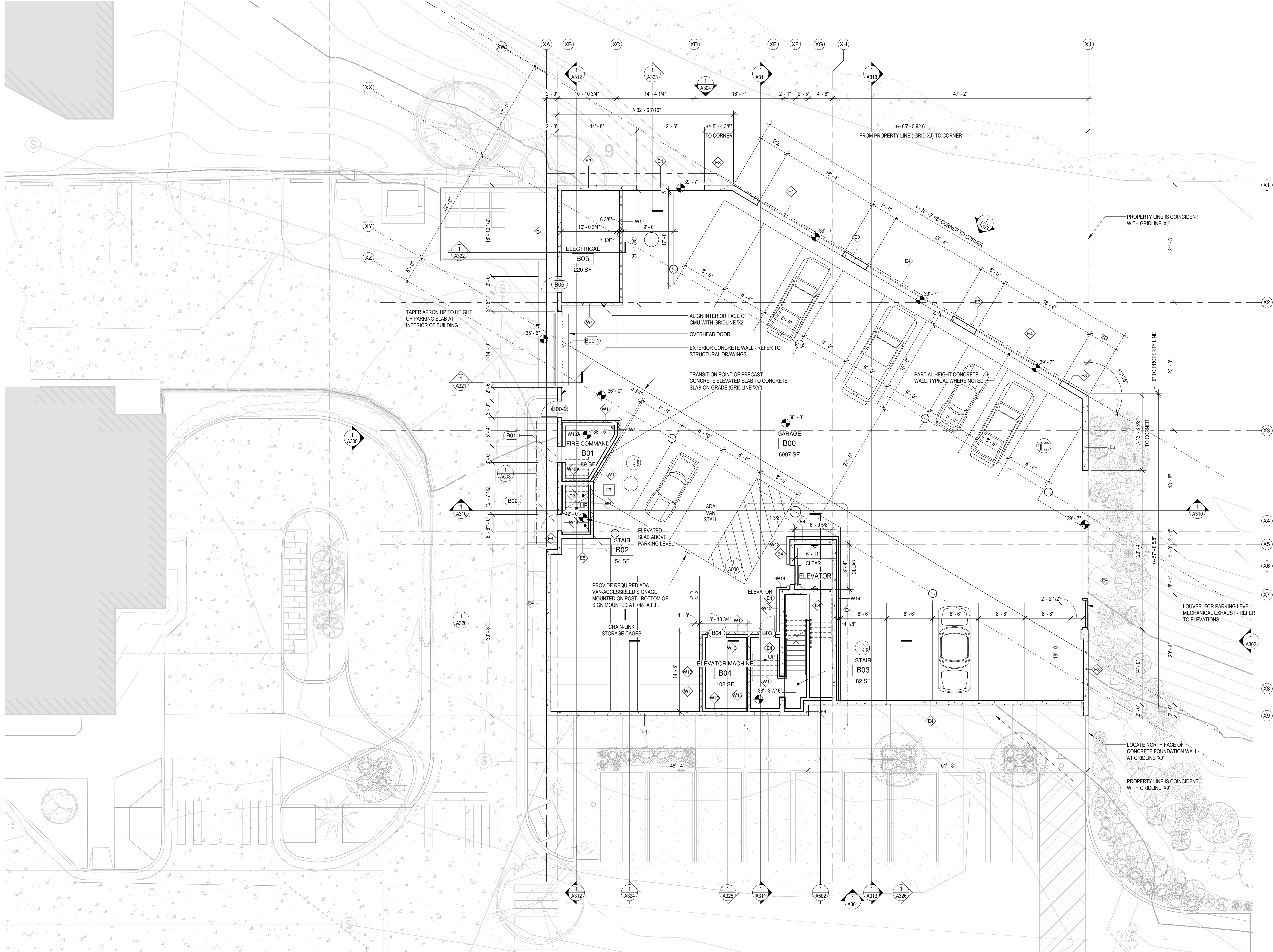
1 Parking Level Floor Plan 1/8" = 1'-0"
